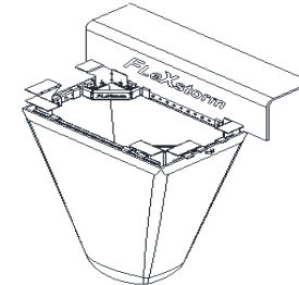
62MCBILT3 & 62MCBILT11 - Curb Box
