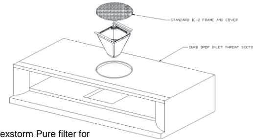
Flexstorm Pure filter for Virginia DI-3
